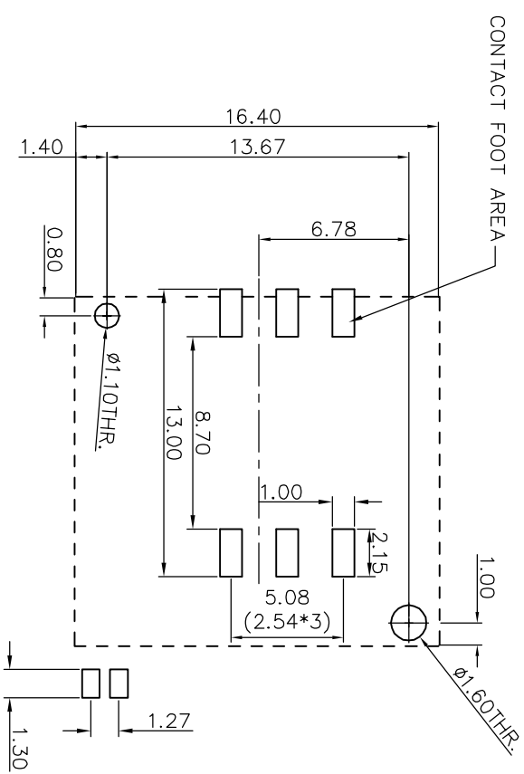
REFERENCE PC BOARD LAYOUT
